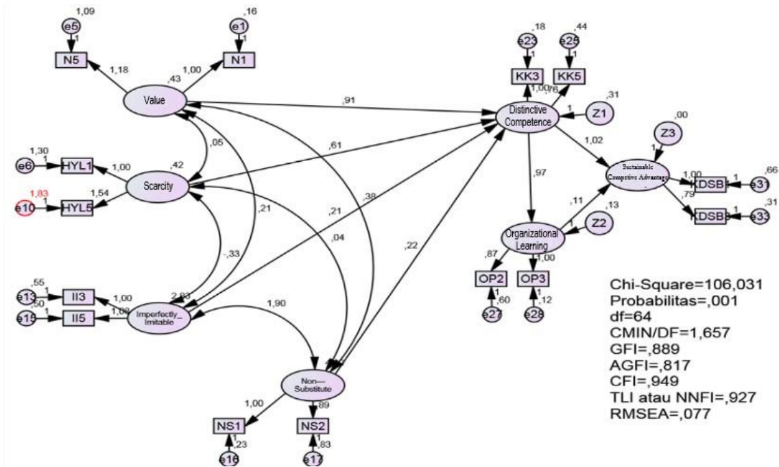
Figure 5. Full Model Fit SEM
