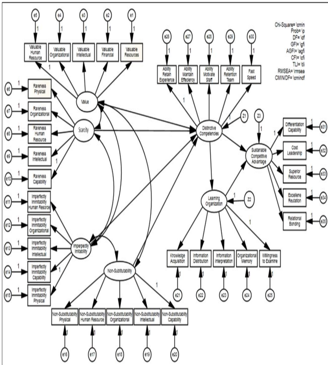
Figure 3. Path Diagram in this Research
