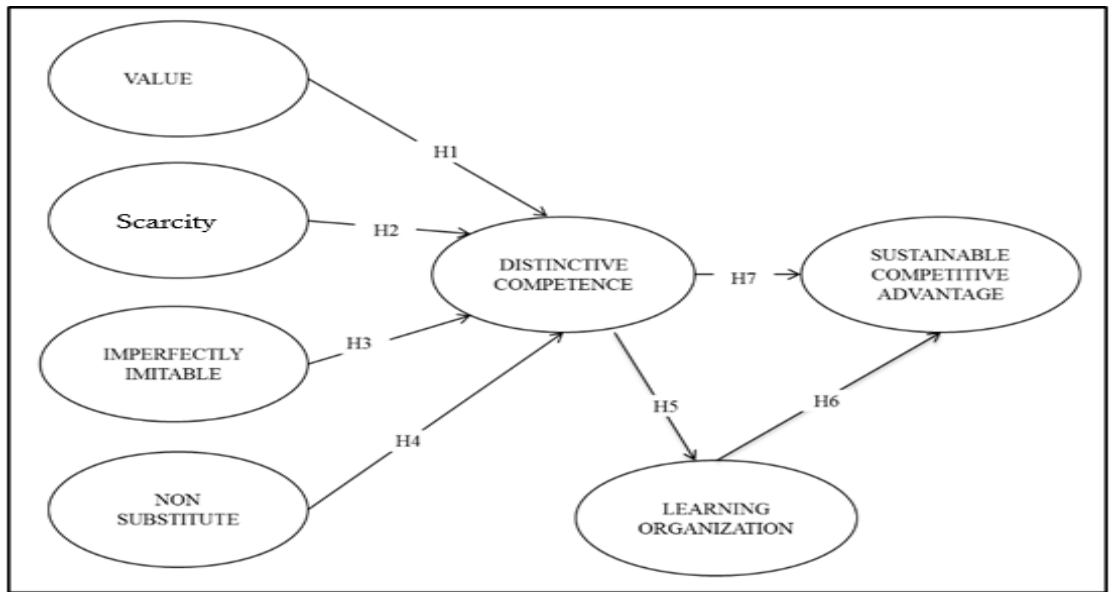
Figure 2. Empirical Research Model
