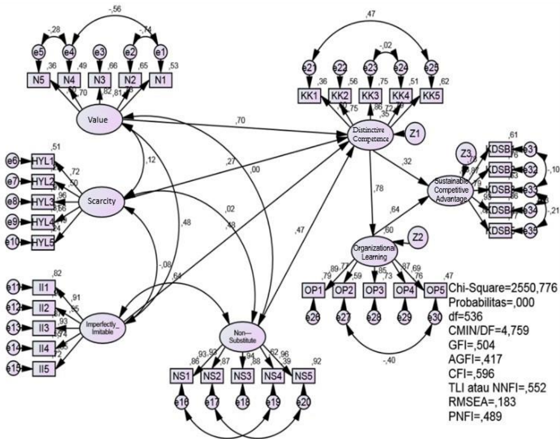
Figure 4. SEM Model Testing
