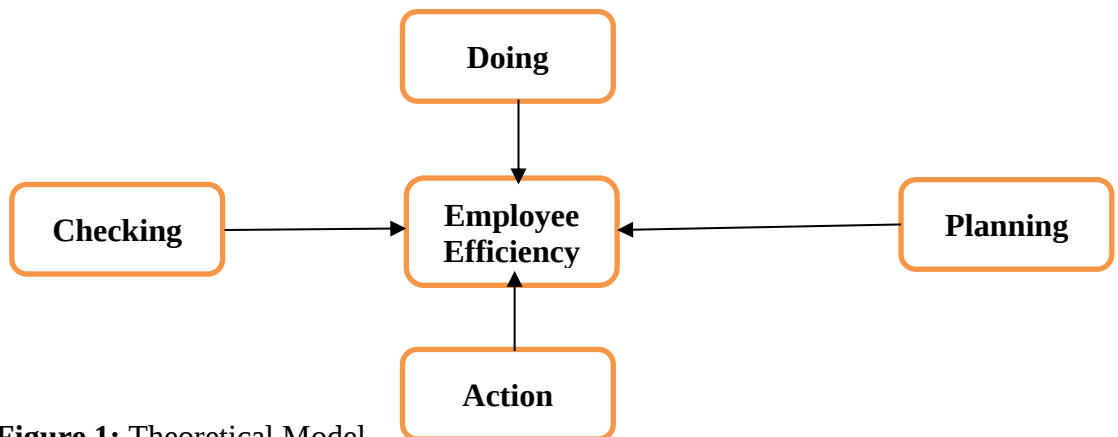
Figure 1: Theoretical Model
